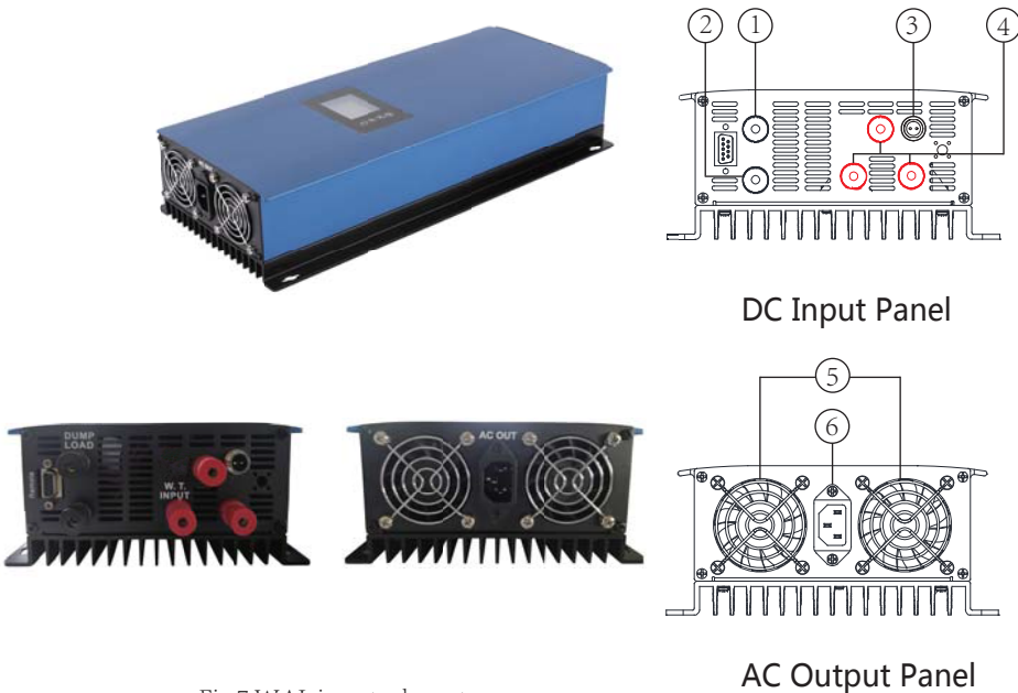
Fig.7 WAL inverter layout
