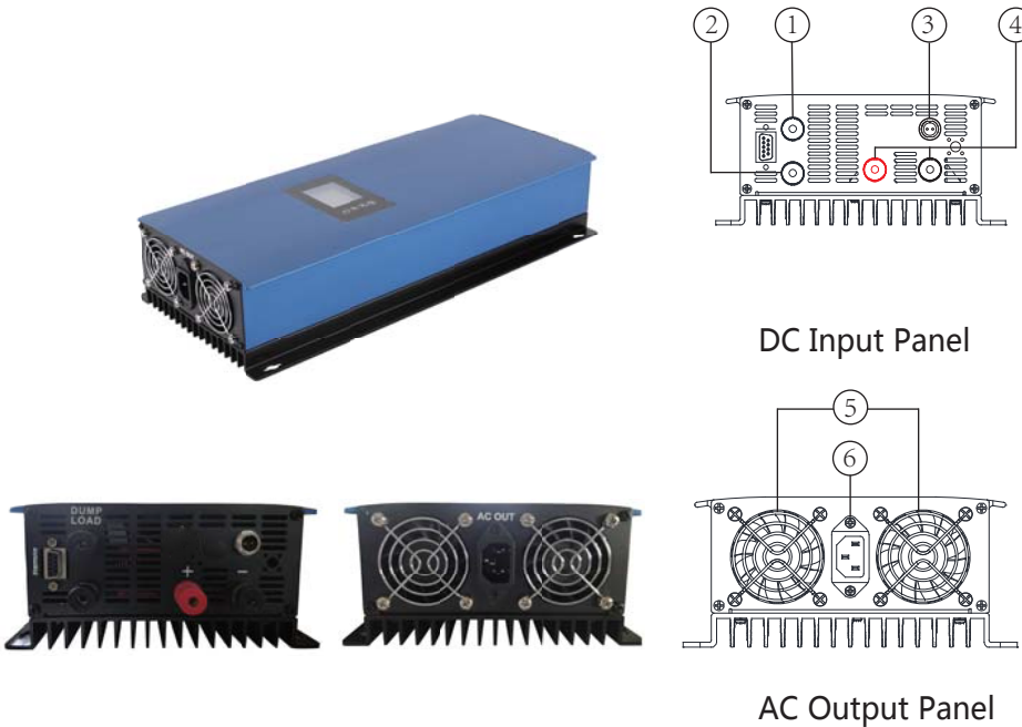
Fig.6 WDL inverter layout
