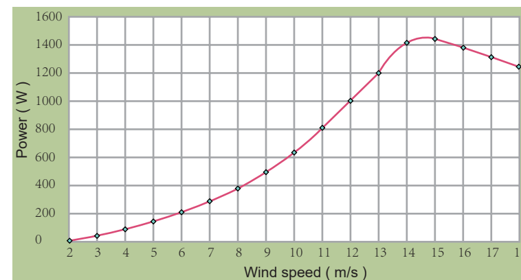
Fig 2.Wind speed--Power Curves
