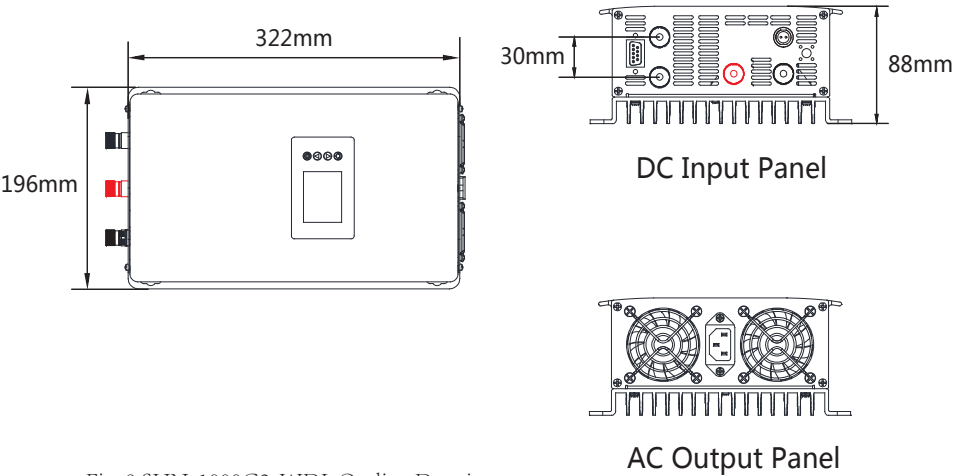
Fig. 9 SUN-1000G2-WDL Outline Drawing
